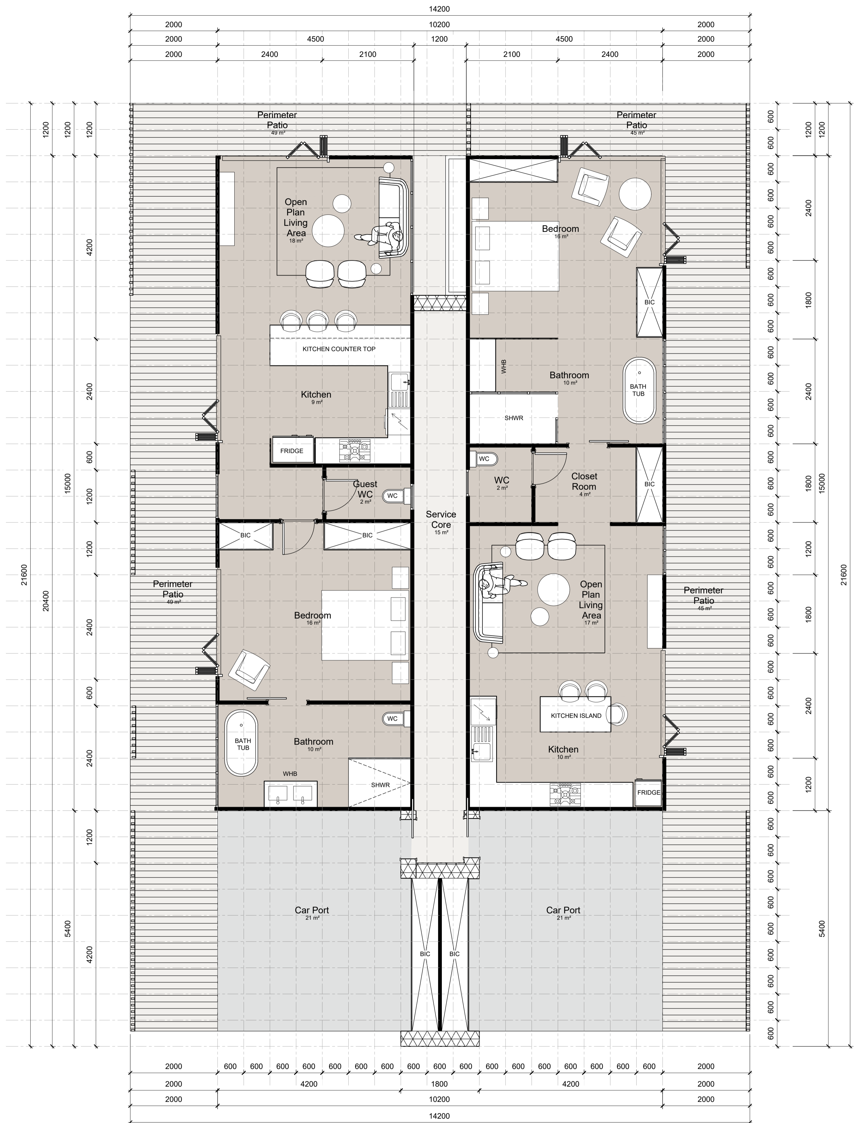
Garden Unit Option 2 + 3 - Two types of one bedroom units Ground Floor Plan 1:50
