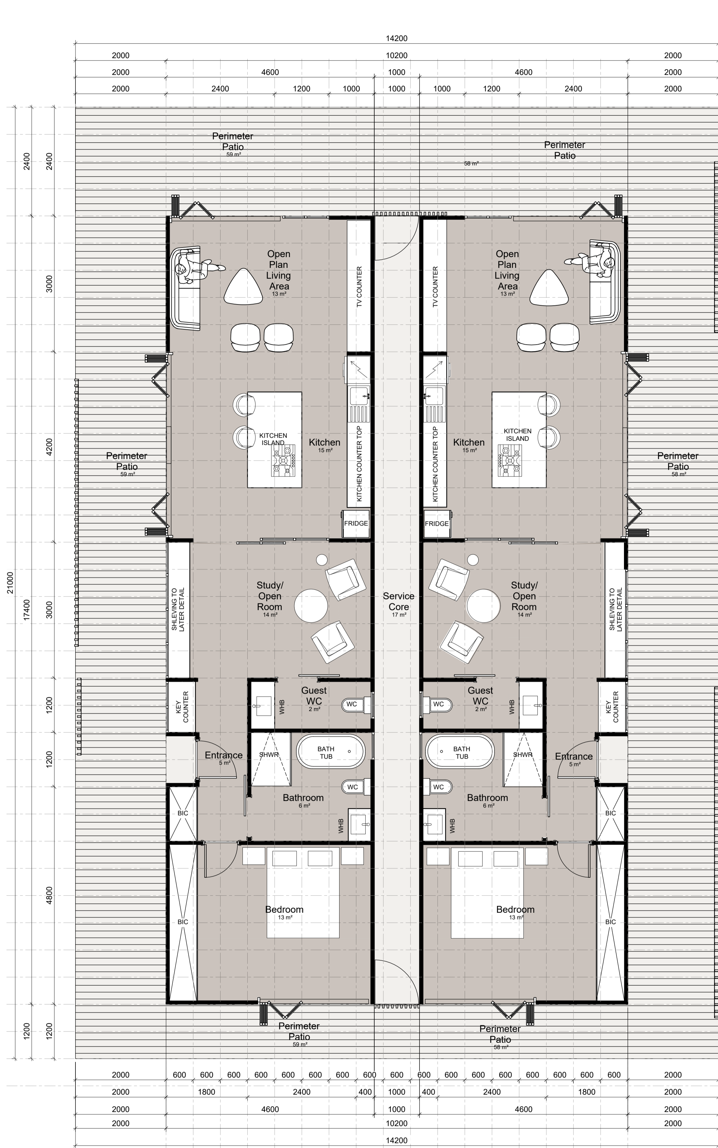
Garden Unit Option 1 - One to two bedroom (study becomes extra bedroom) unit Ground Floor Plan 1:50
